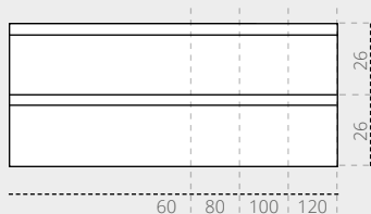
Onderkast 2 laden symmetrisch met opliggende fronten gefreesd / Washbasin cabinet 2 drawers symmetrical with straight-up front milled 60 / 80 / 100 / 120 x 46 x 52 cm
